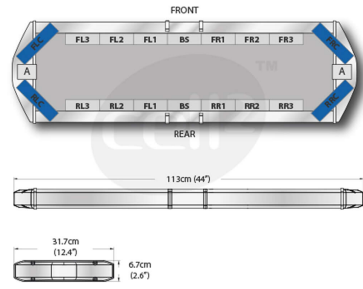
TOP OF LIGHTBAR
